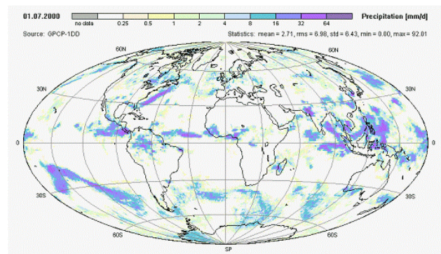
Figure 14. GPCP-1DD multi-satellite estimates of precipitation (mm) for July 01, 2000.
