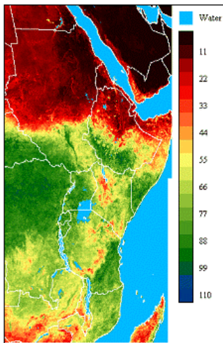
Figure 15. Relative evapotrans- piration from METEOSAT - May 2002
