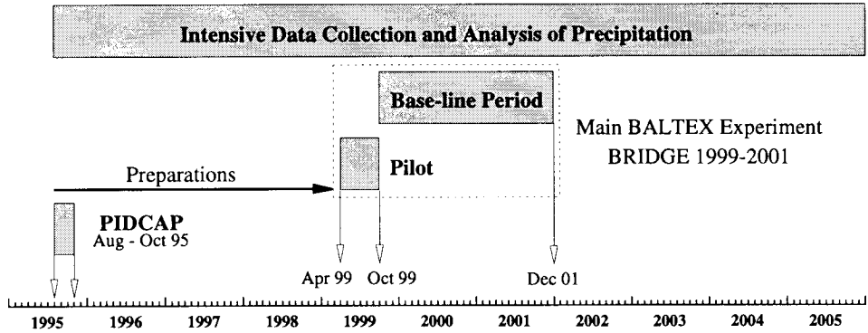
Fig. 7. Time-line for BRIDGE related precipitation analysis. The period of intensive data collection and analysis of precipitation beginning with PIDCAP is at present foreseen to be executed during October 1999 to December 2001 and to extend to at least 2005. At the end of 2005 more than 10 years of daily precipitation fields based on more than 4,200 corrected rain gauge observations within the Baltic Sea drainage basin will be archived in the data base of the BMDC.
