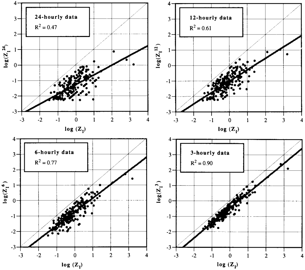
Fig. 3. Precipitation intensities \log(Z_I^n) calculated from 24-, 12-, 6- and 3-hourly sums vs. precipitation intensity \log(Z_I) , based on hourly observations from 14 automatic weather stations GEONOR T200 during the 92 days of the PIDCAP period. Units in mm/h.
