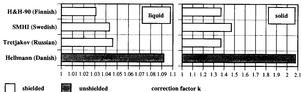
Fig. 1. Aerodynamic correction factors for the predominantly used gauge types in the Baltic Sea Drainage Basin. Mean values for Jokioinen, Finland, based on the field experiment 1987-1993 (after F rland et al. 1996).
